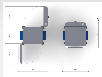
Topview Label Inspector opened/closed
